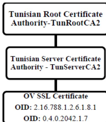
Figure 1- TunRootCA2 hierarchy
